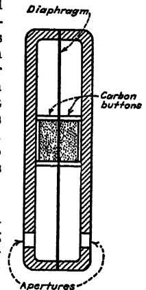
Cross-section of lip microphone.
